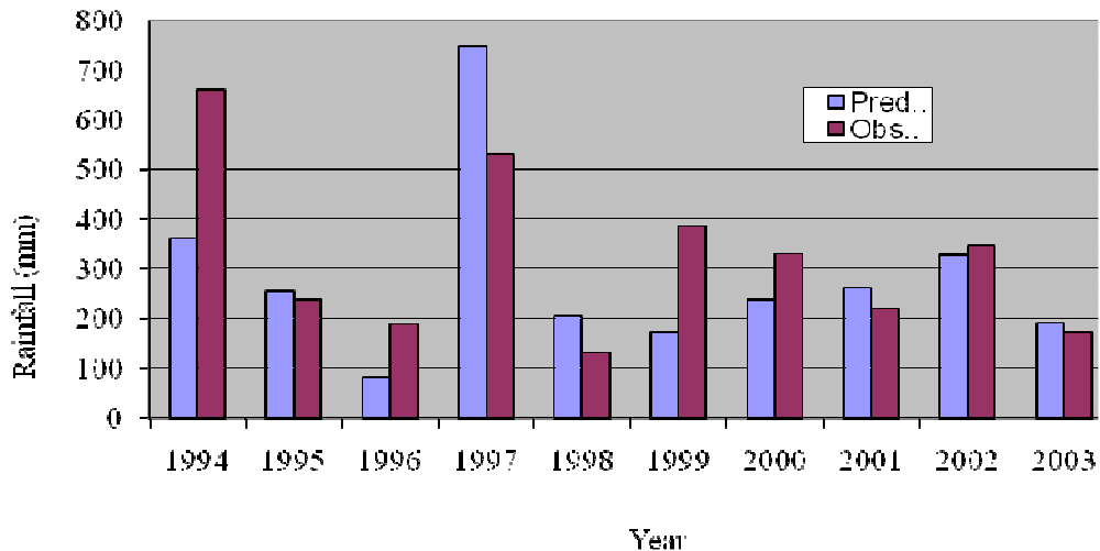
Figure 1. Predicted and observed amounts of rainfall (September-November), 1994 to 2003. Source: Katumani Meteorological Station.
